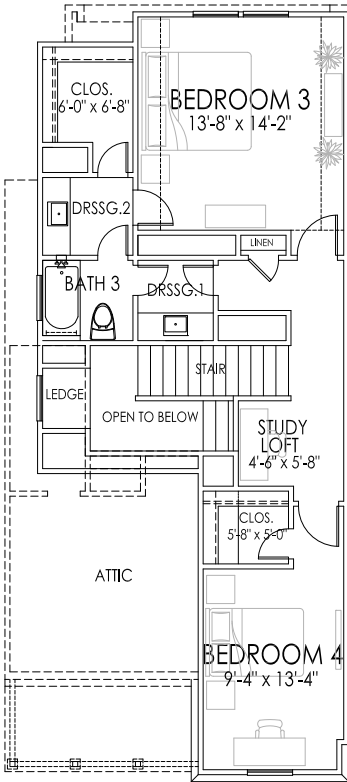
THIRD FLOOR
