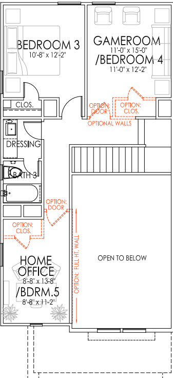
THIRD FLOOR
