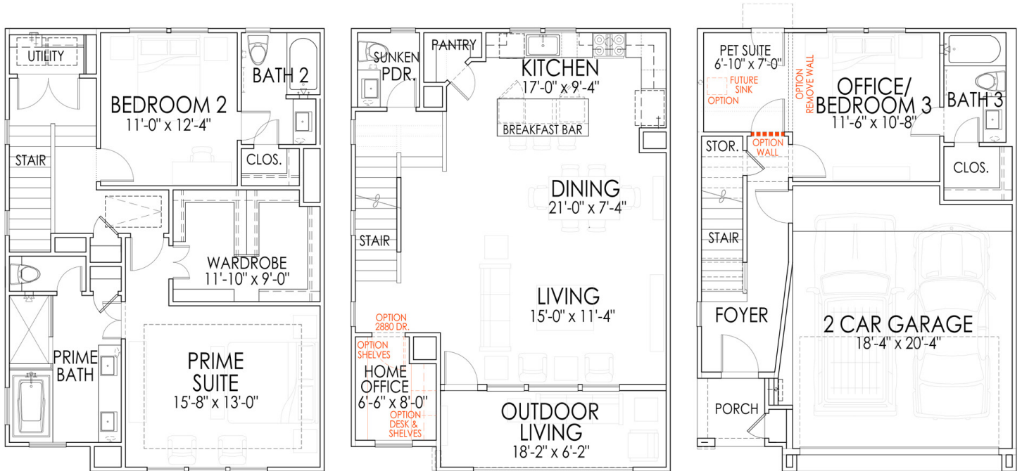
THIRD FLOOR
