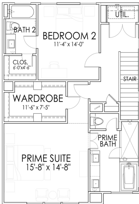
THIRD FLOOR
