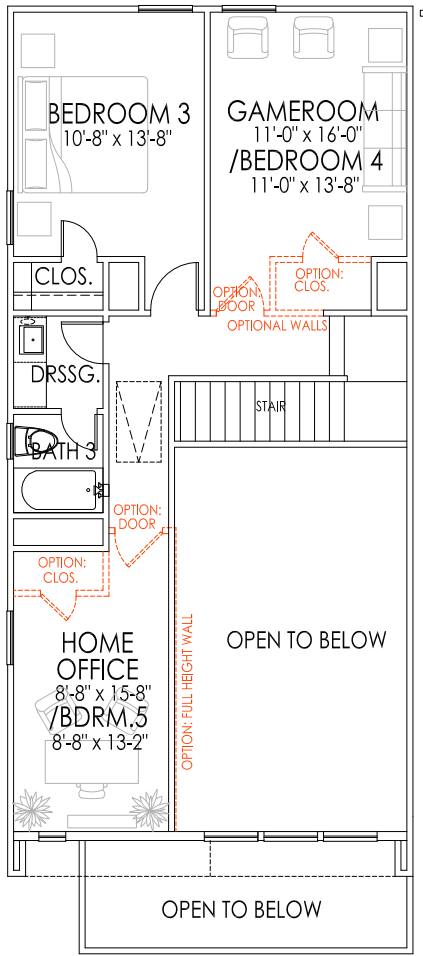
THIRD FLOOR
