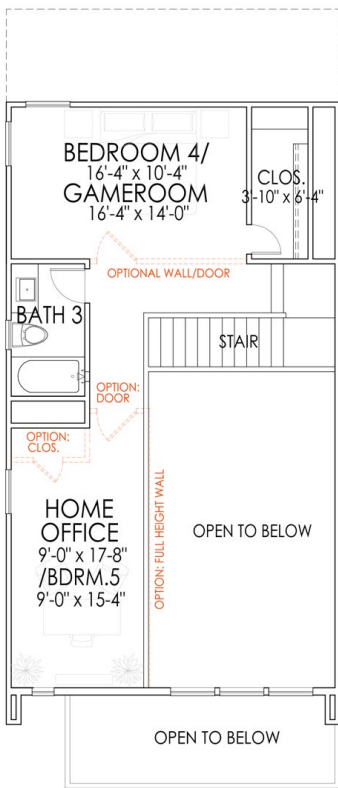
THIRD FLOOR
